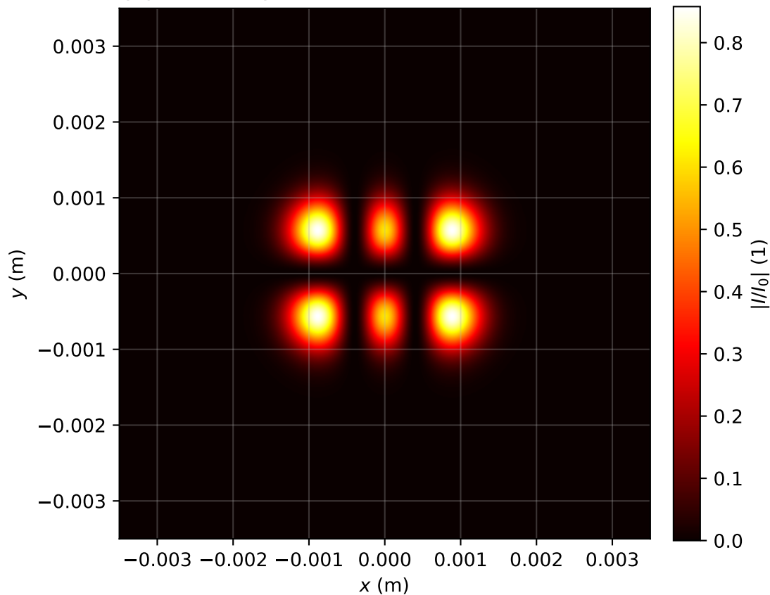
Intensity profile I(x, y, z = 1.035)/I_0 , P_{in}=0.5P_{cr} , artificial time
